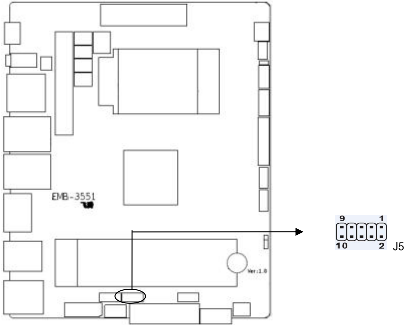
J5: LVDS 固件更新, 2X5PIN 2.0mm 排针
