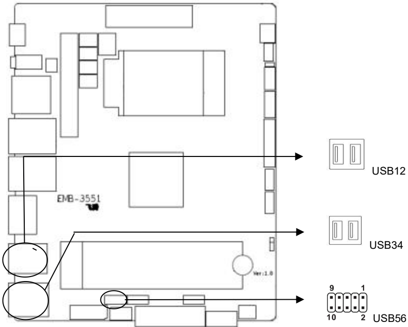
USB56: 2X5PIN 2.0mm 排针
